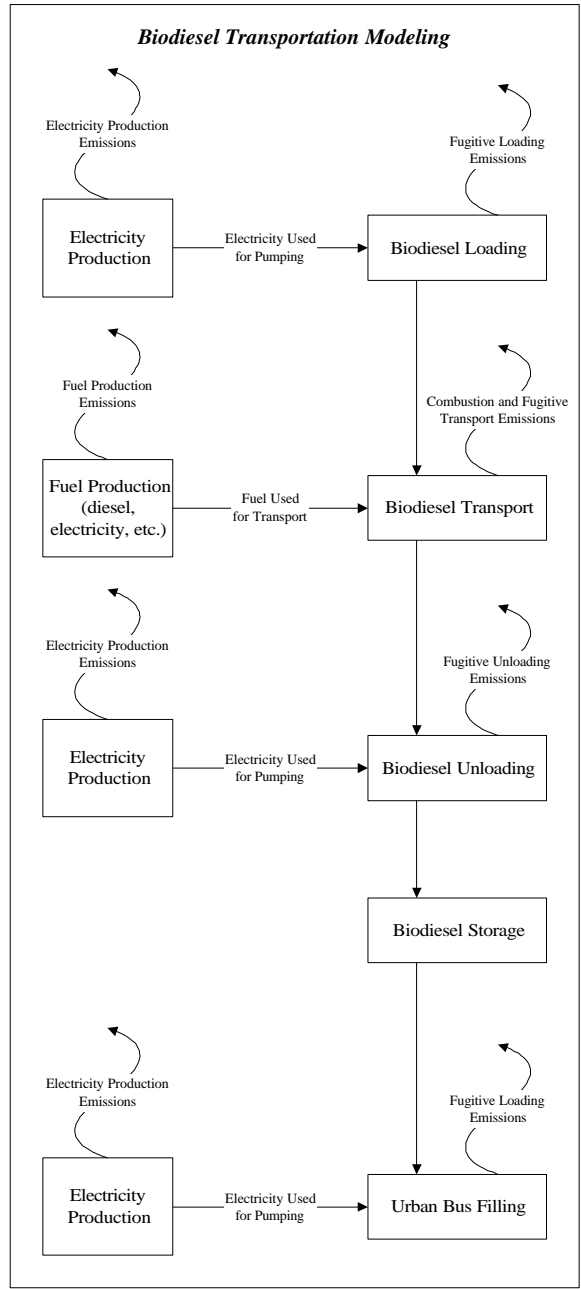
Figure 75: Biodiesel Transportation Modeling
